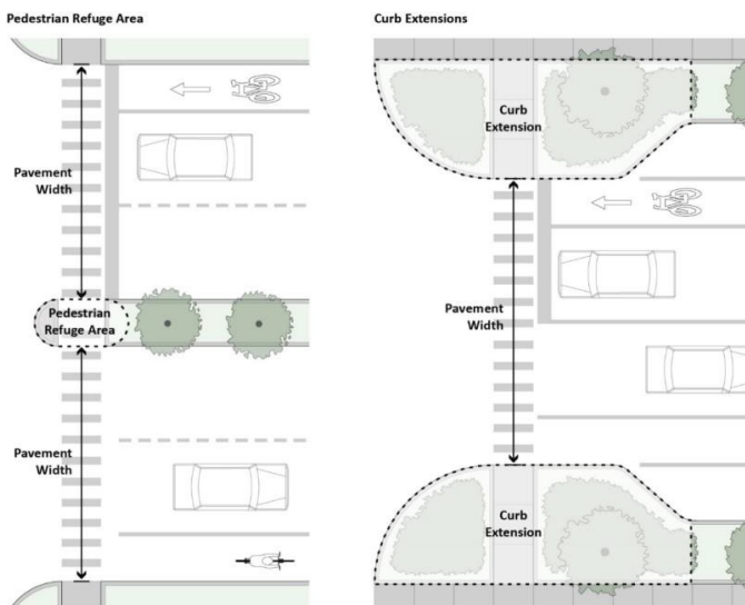
Figure XXXX Pedestrian Crossing Distances
